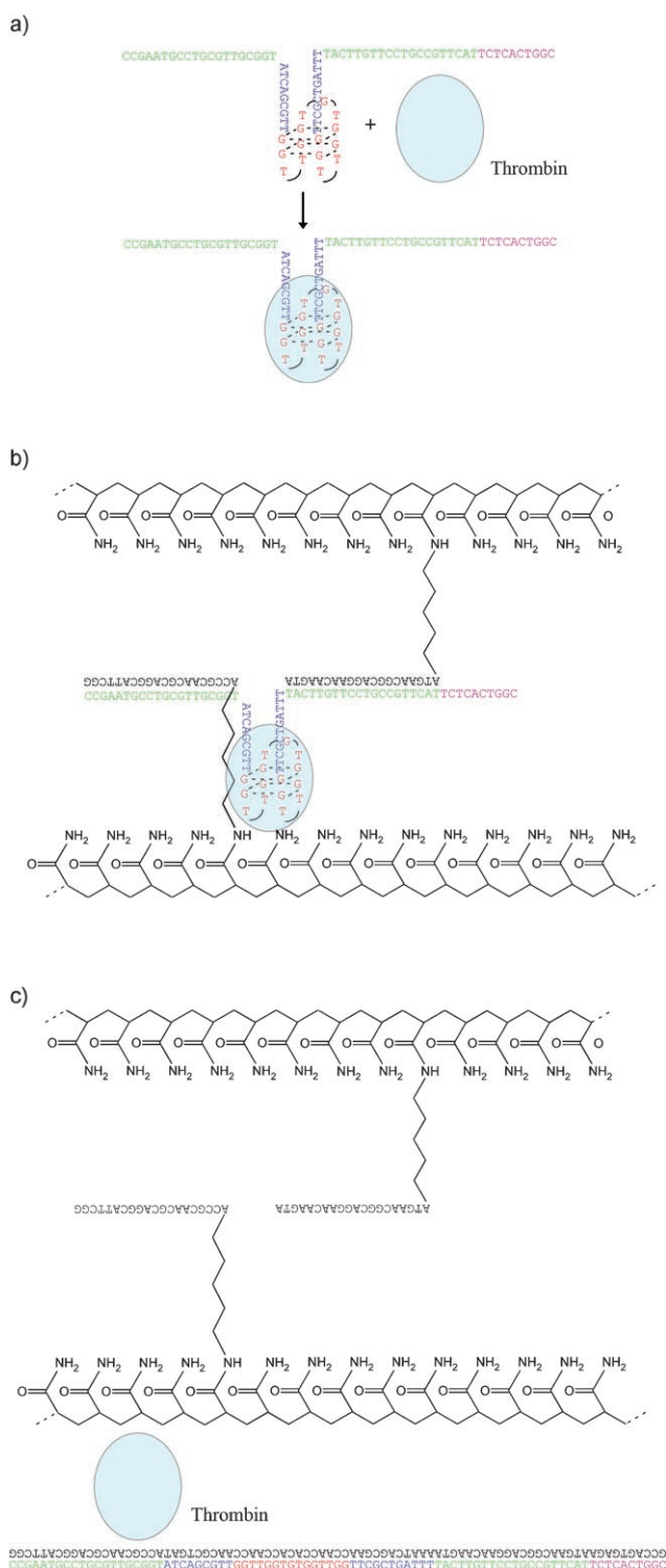
Scheme 1. Capture and release of thrombin by a sol–gel transition.
